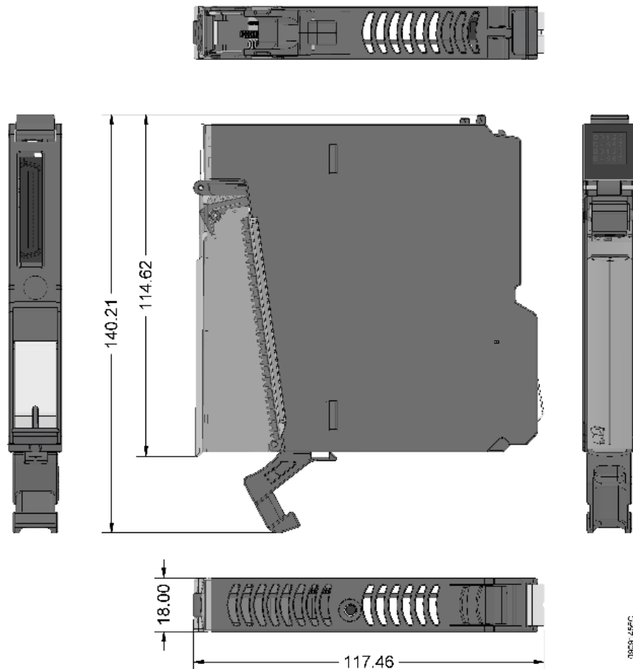
Figure 1: Physical Dimensions
