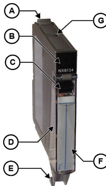
Figure 2: NX6134
