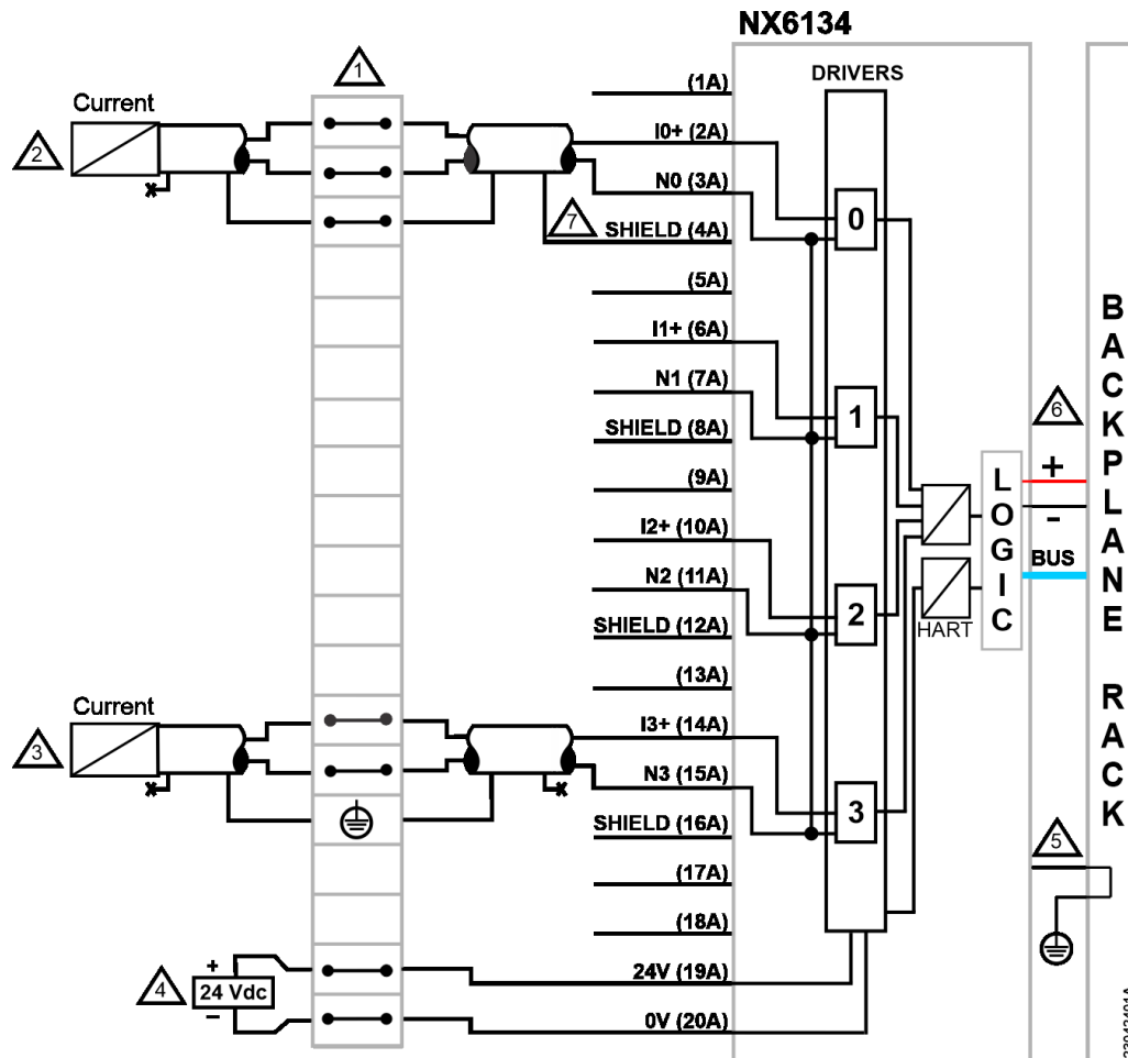
Figure 3: Electric Diagram
