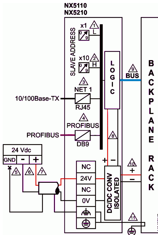
Figure 6: Electrical Diagram
