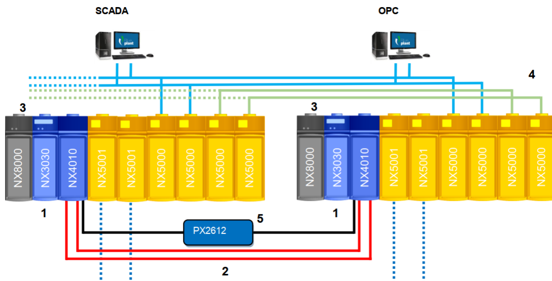
Figure 1: Half-Cluster Redundancy
