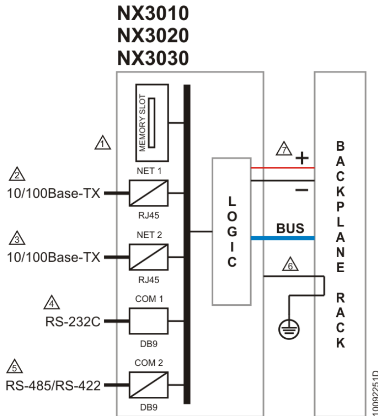
Figure 4: Electrical Diagram of NX-ERA Series NX3010, NX3020 and NX3030 CPUs
