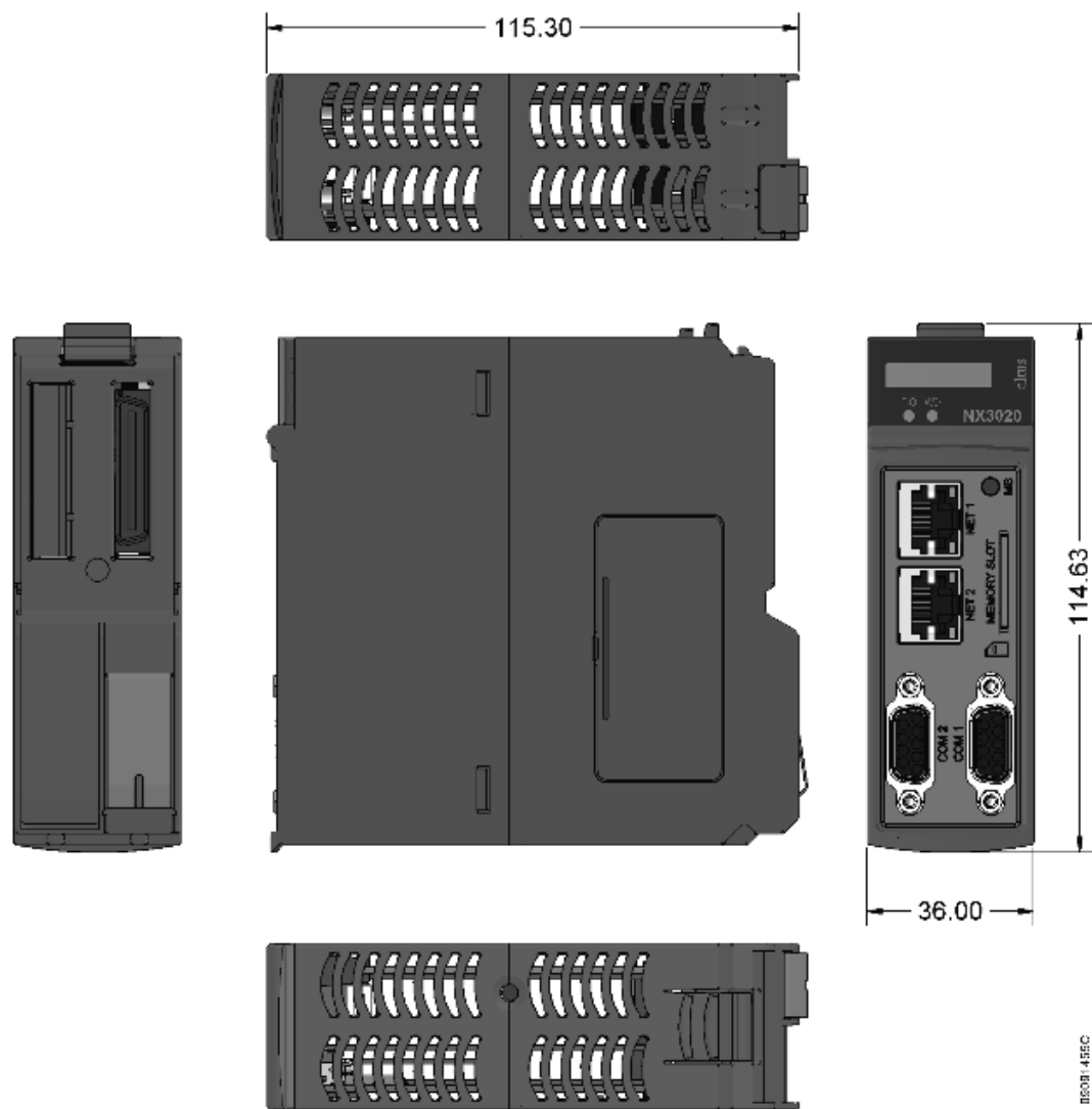
Figure 2: CPU Physical Dimensions
