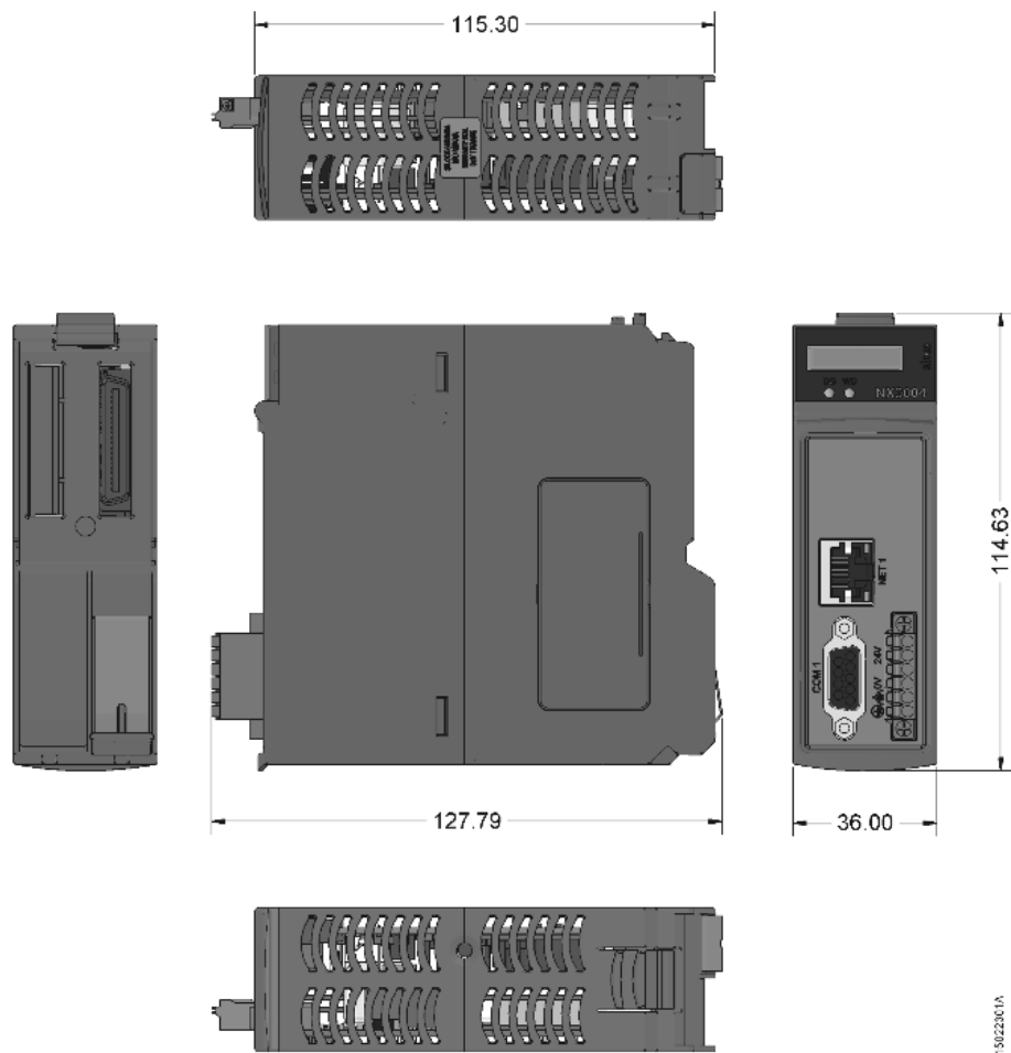
Figure 1: NX3004 and NX3005 CPU Physical Dimensions
