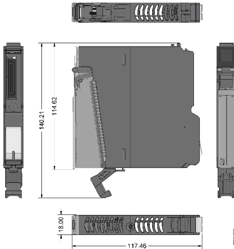
Figure 1: Physical Dimensions
