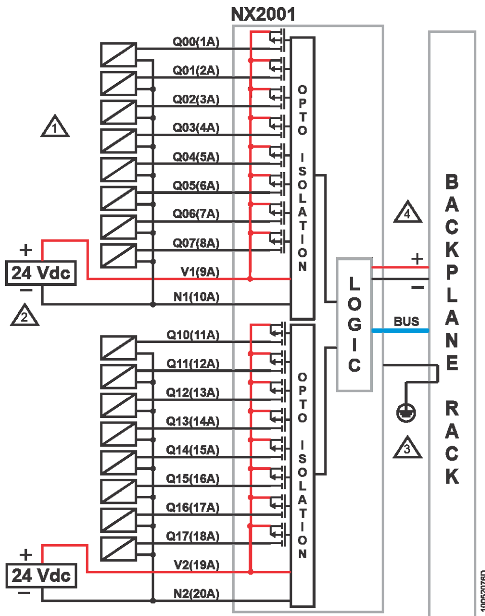
Figure 3: Electric Diagram
