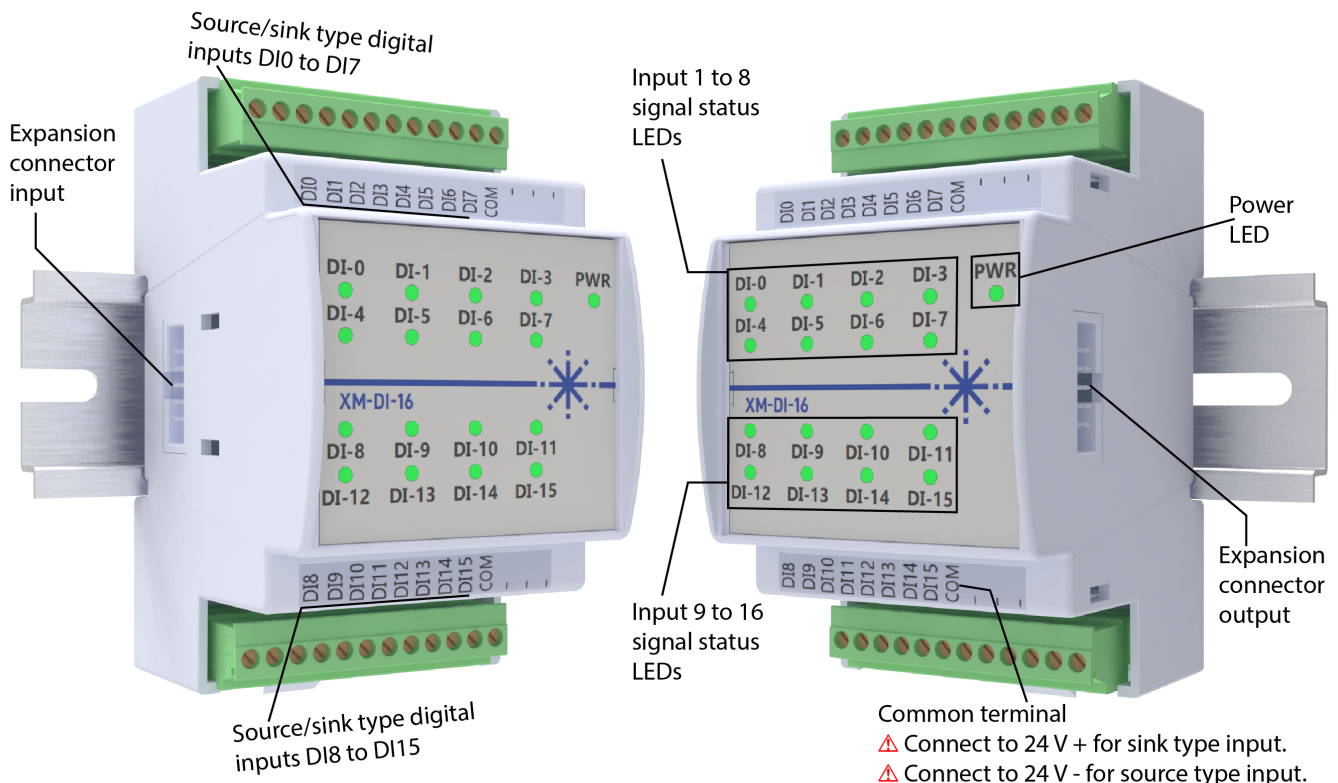
Figure 1. XM-DI-16 Digital Output Expansion Module
